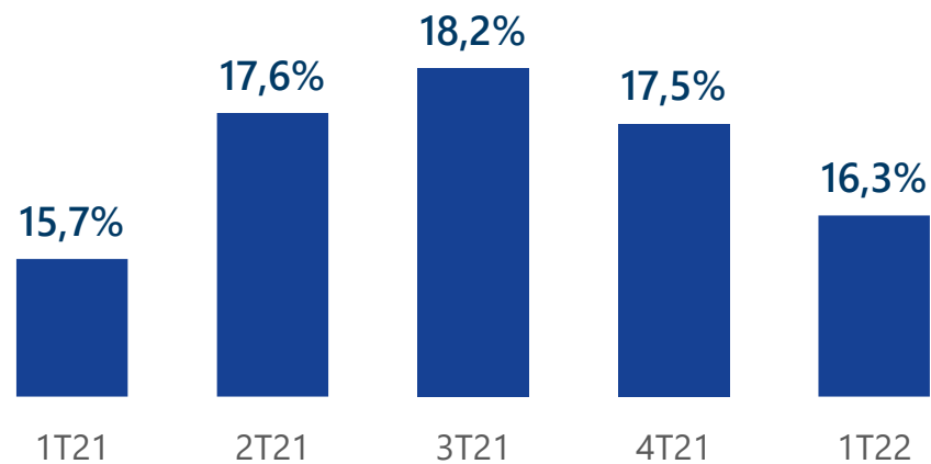
ROAE (1) (a.a) (%)
